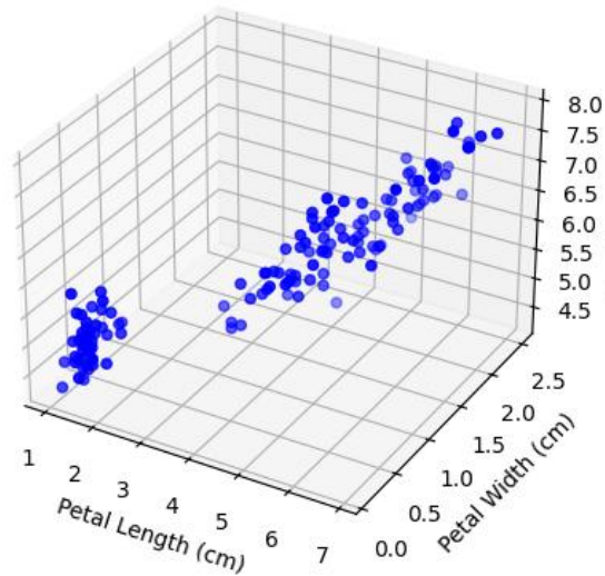
Bivariate Regression
